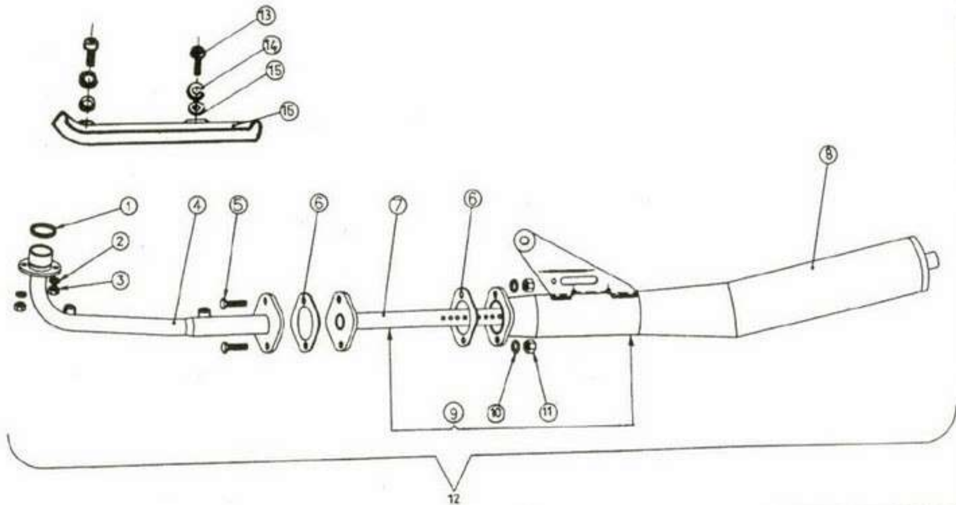
SILENCER ASSEMBLY
