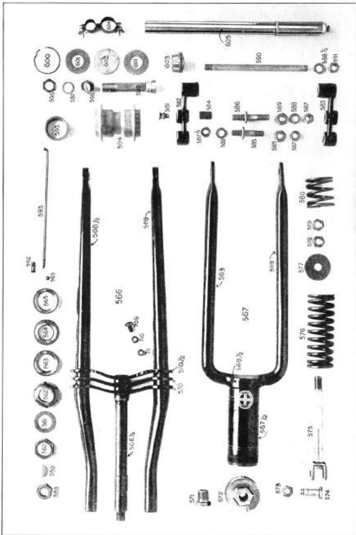
IX—FORK AND FRONT WHEEL PARTS
