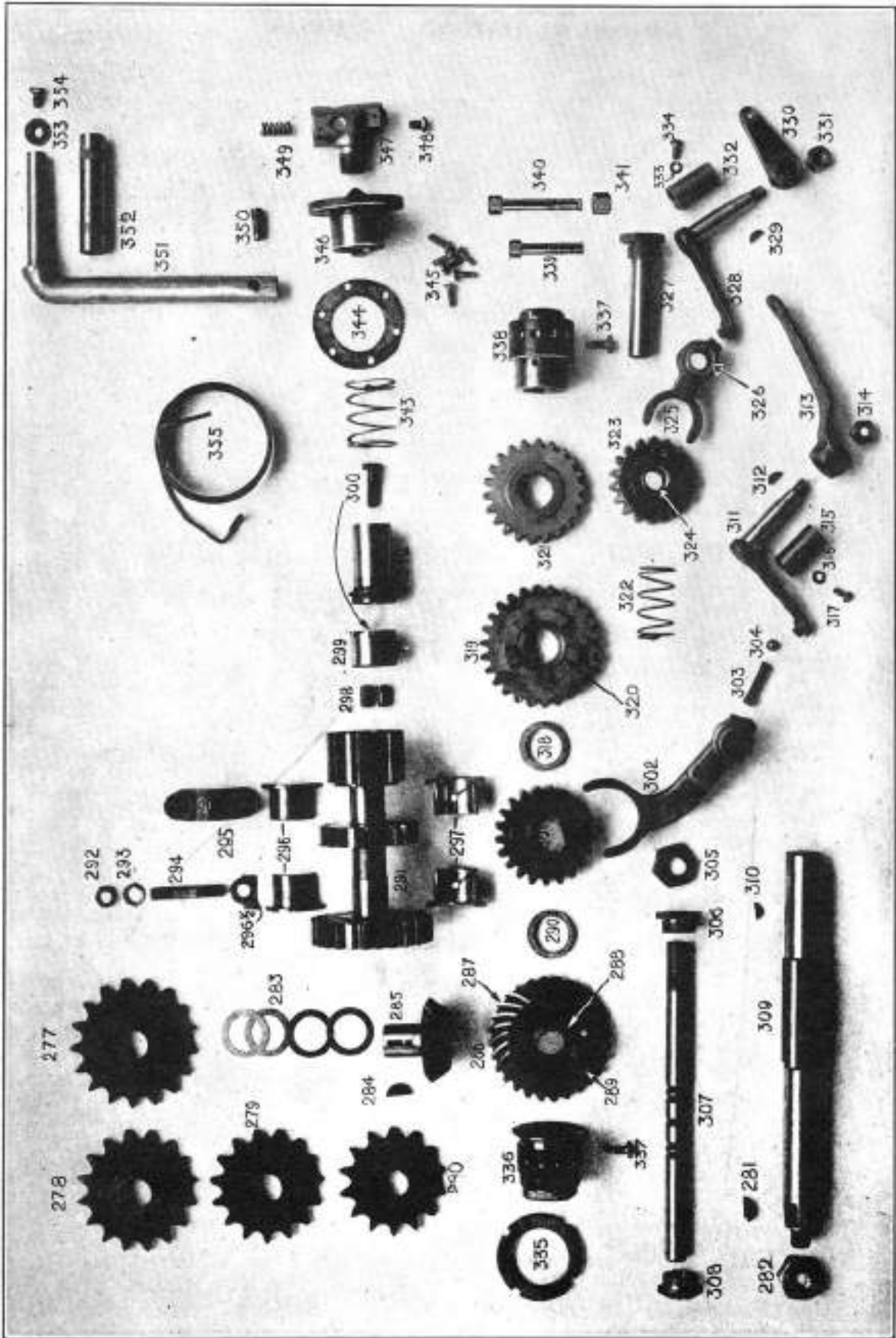
V-TRANSMISSION PARTS
