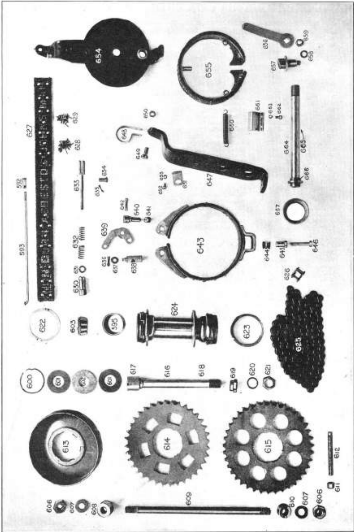
X—BRAKE AND REAR WHEEL PARTS
