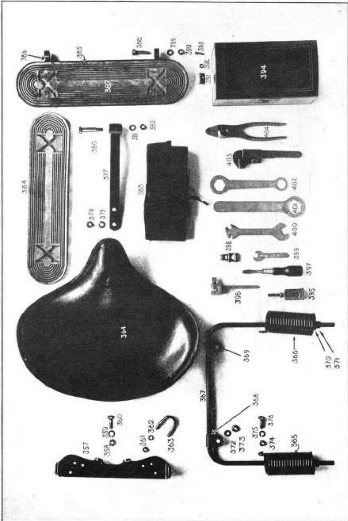
VI—SADDLE, TOOL KIT AND FOOT BOARDS
