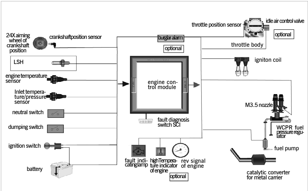
Structural drawing of EFI system
